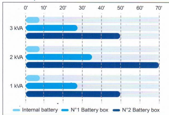
Back up time for Tower UPS
