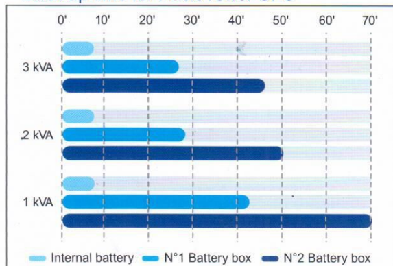
Back up time for Rack/Tower UPS
